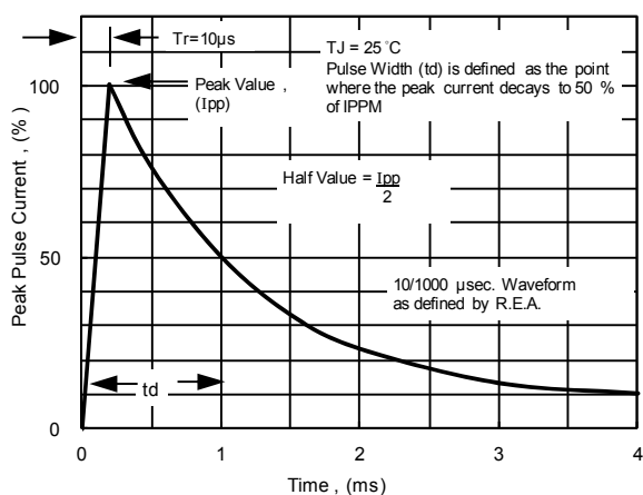
Fig. 5 - Pulse Waveform
